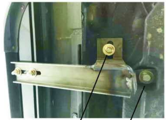
Rear Bracket Mounting Position
